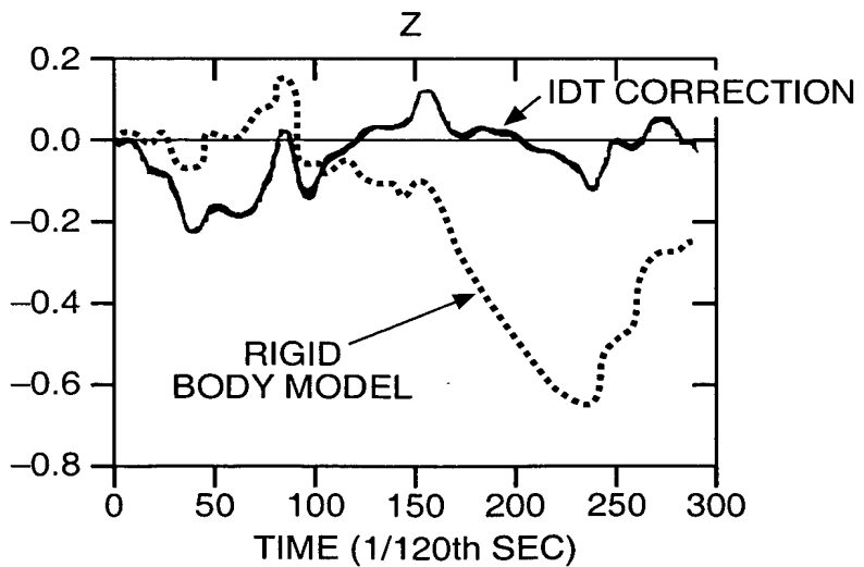
DISPLACEMENT (cm) FIG. 16C
